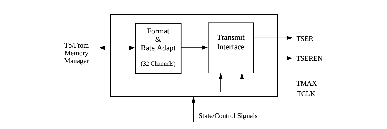
Figure 5. Block Diagram of Transmit Bit-Level Processor
