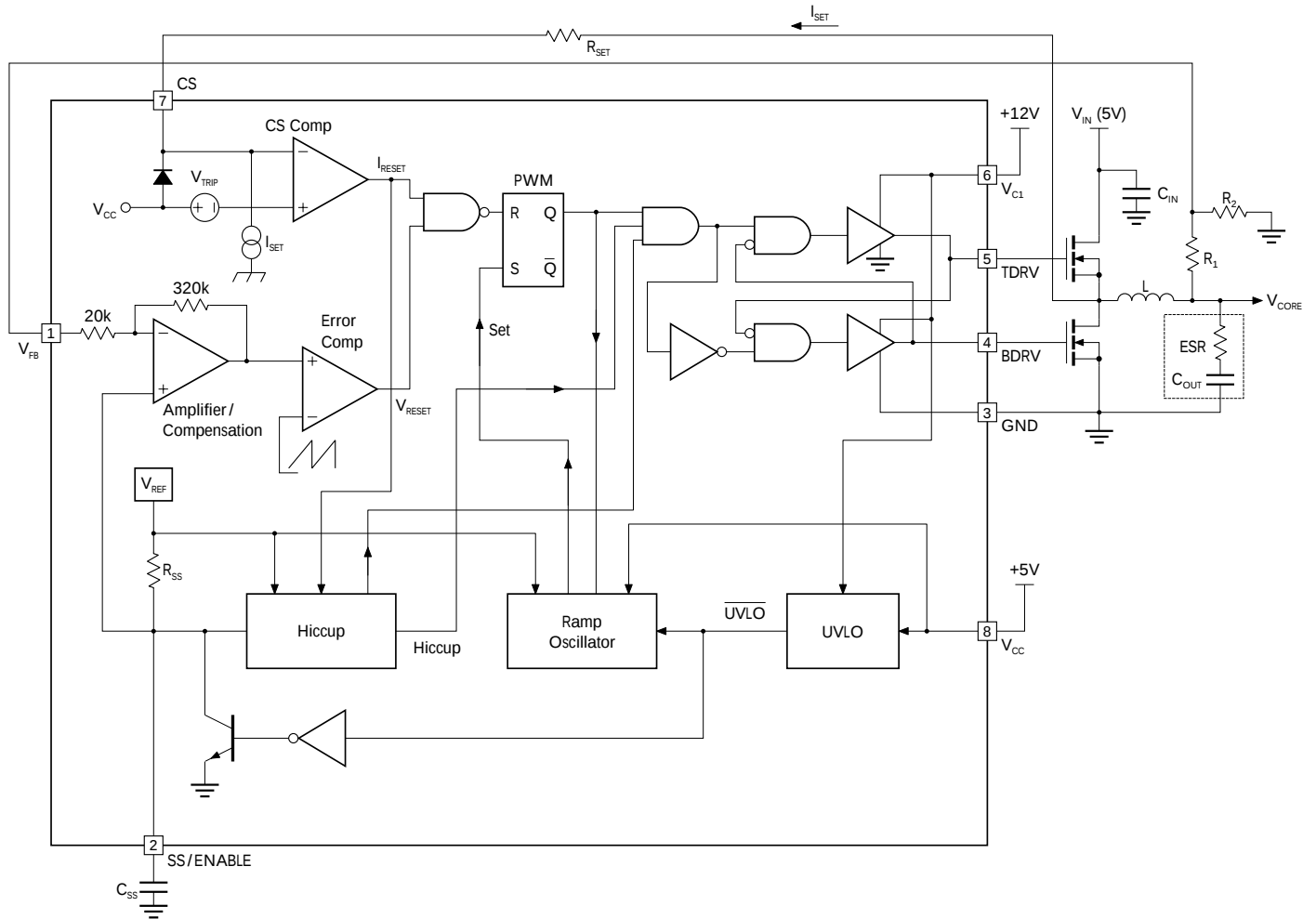
FIGURE 1 — Block Diagram
