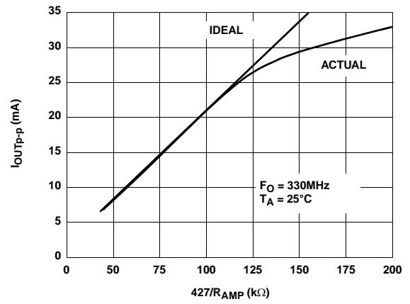
FIGURE 4. I_{OUTp-p} vs 427/R_{AMP}
