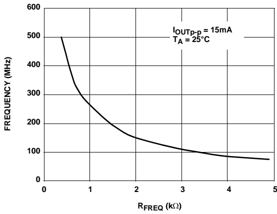
FIGURE 1. FREQUENCY vs R_{FREQ}
