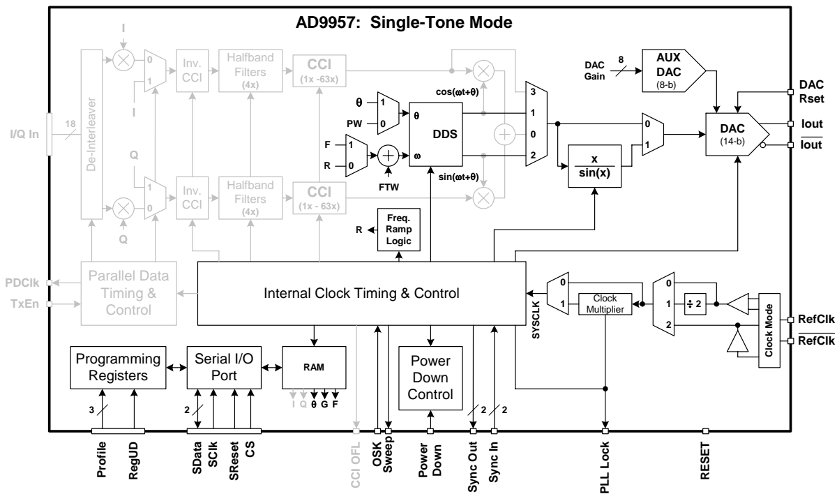
Figure 13: Single-Tone Mode
