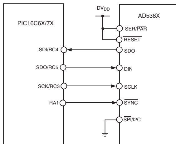
Figure 16. AD5380-PIC16C6X/7X Interface
