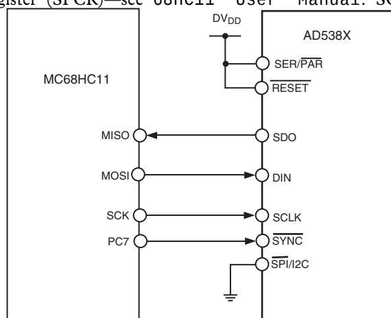
Figure 15. AD5380-MC68HC11 Interface
