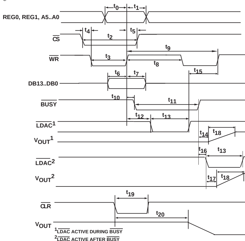
Figure 6. Parallel Interface Timing Diagram
