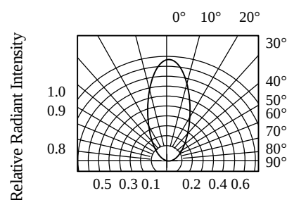
FIG.6 RADIATION DIAGRAM
