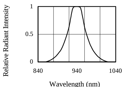
FIG.1 SPECTRAL DISTRIBUTION
