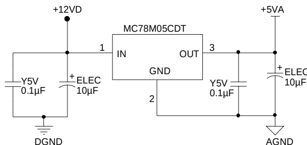
Figure 15. Voltage Regulator
