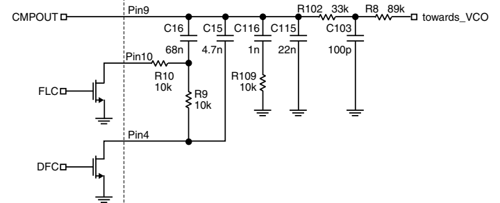
Figure 7. Dual-Loop Filters
