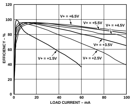
Figure 6. Power Efficiency vs. Load Current
