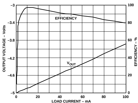
Figure 2. Output Voltage and Efficiency vs. Load Current
