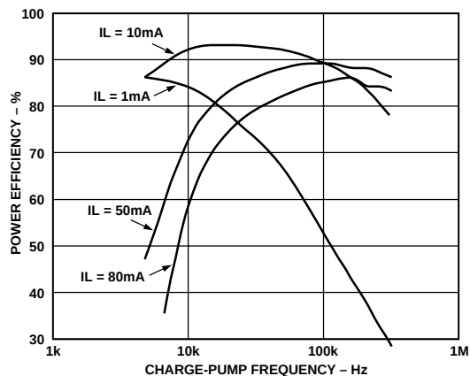
Figure 4. Efficiency vs. Charge-Pump Frequency
