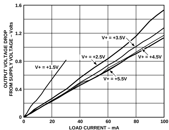
Figure 3. Output Voltage Drop vs. Load Current
