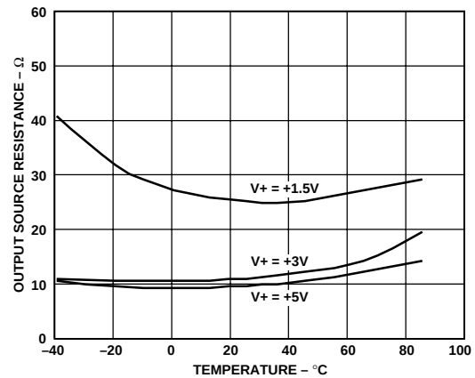
Figure 14. Output Resistance vs. Temperature
