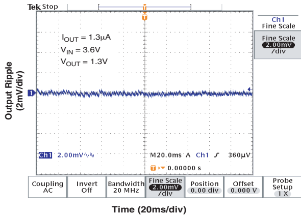
Output Ripple
