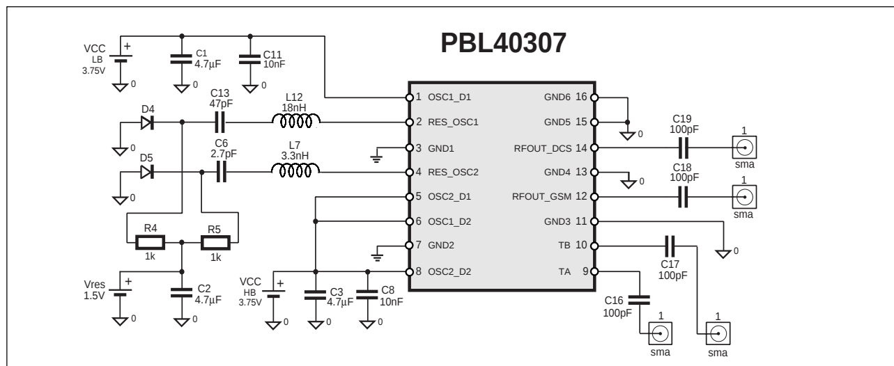
Figure 3. Evaluation Board schematic.
