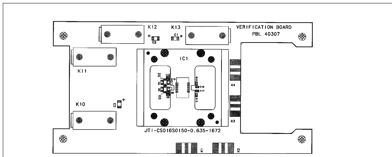
Figure 4. Evaluation Board layout.
