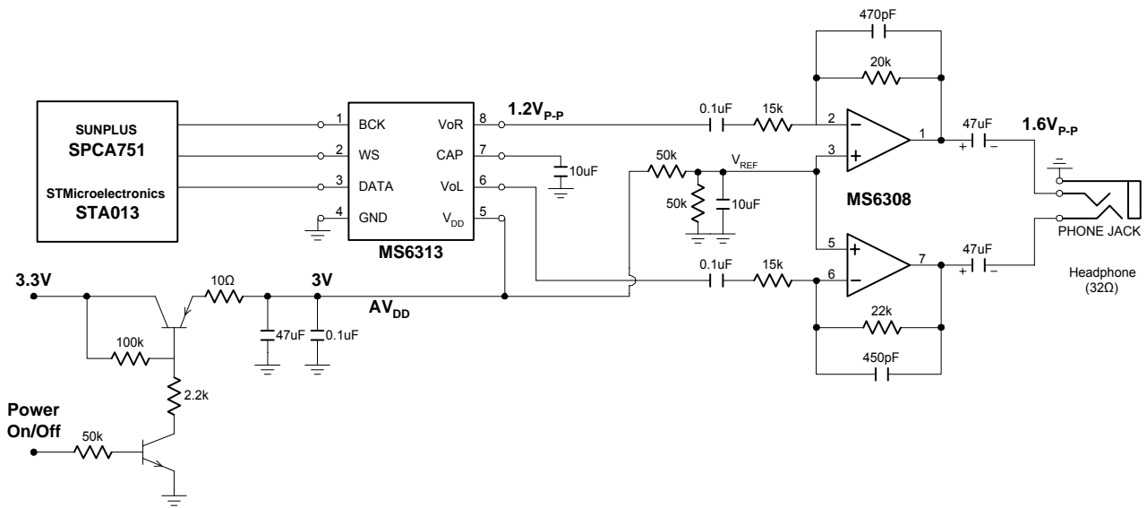
Fig.6 A first order lowpass filter for DAC output.
