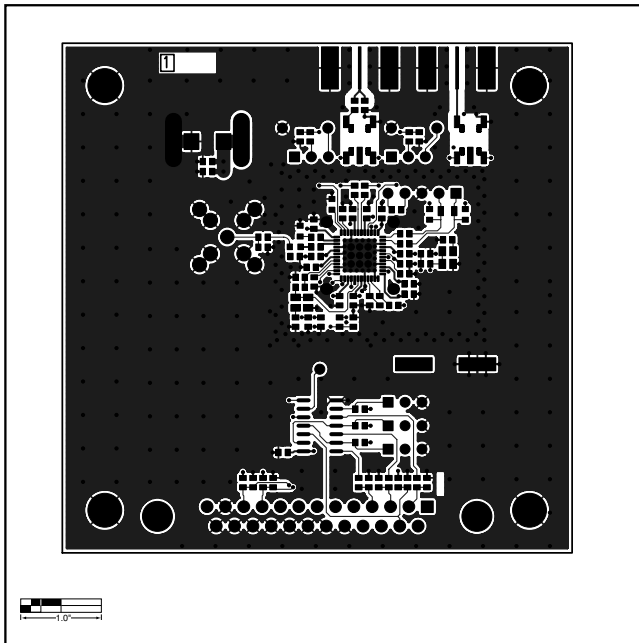
Figure 5. MAX355x EV Kit PCB Layout—Primary Component Side
