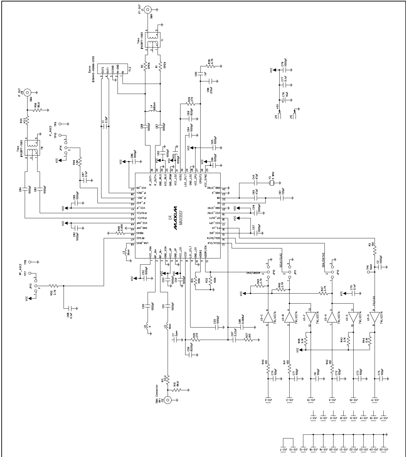
Figure 1. MAX355_EV Kit Schematic (Sheet 3 of 3)
