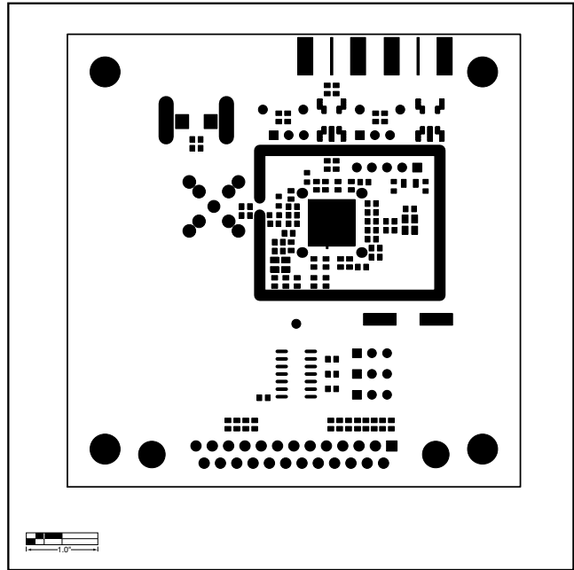
Figure 4. MAX355x EV Kit PCB Layout—Top Soldermask
