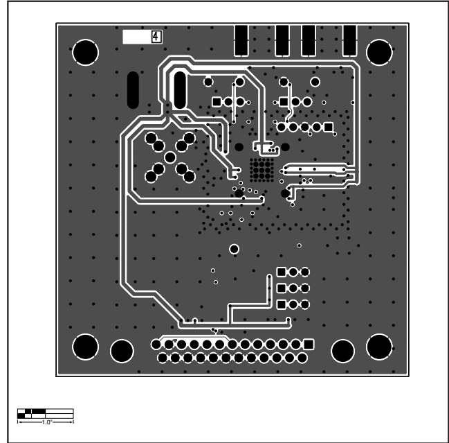
Figure 8. MAX355X EV Kit PC Board Layout—Secondary Component Side
