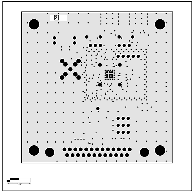
Figure 6. MAX355x EV Kit PCB Layout—Inner Layer 2
