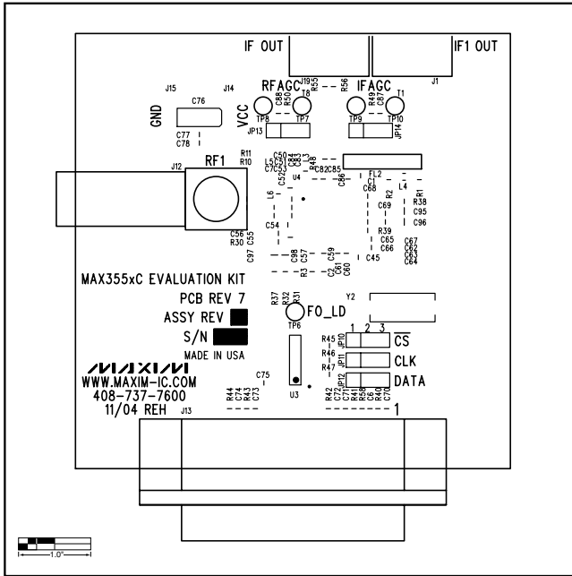
Figure 3. MAX355x EV Kit PCB Layout—Top Silkscreen
