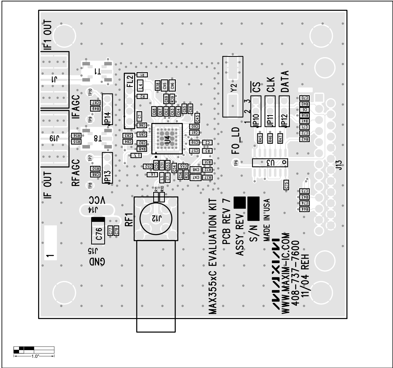
Figure 2. MAX355x EV PCB Layout—Component Placement Guide
