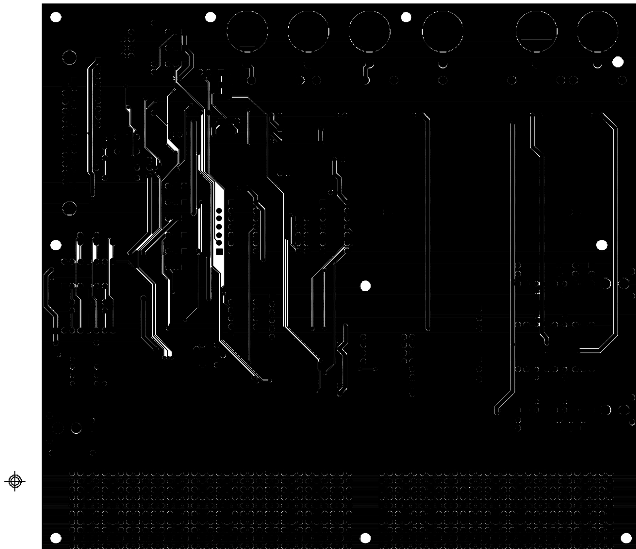
Figure 13. Bottom Side
