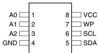
8-lead PDIP
