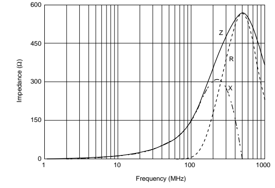
BLM18BB151SN1
