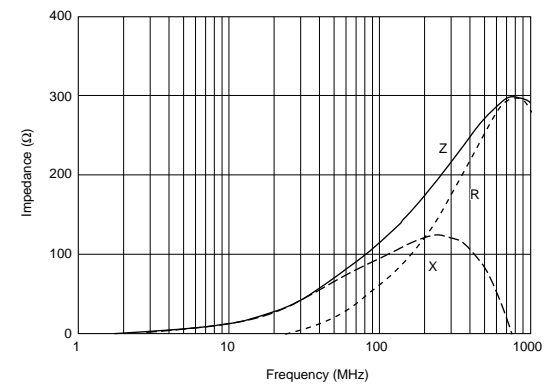
BLM18BD121SN1
