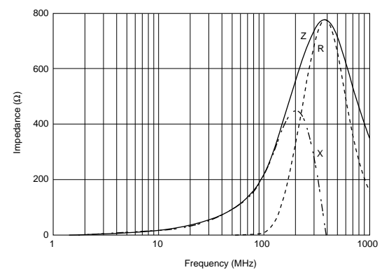
BLM18BB221SN1
