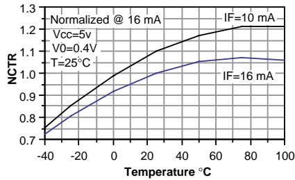
Figure 9. NCTR vs. temperature (SFH6316T/43T)
