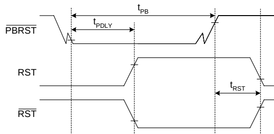
Pushbutton Reset
