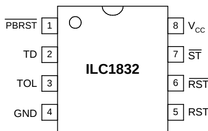
ETC1832N - 8 Lead Plastic DIP Package ETC1832M - 8 Lead Plastic SOIC Package
