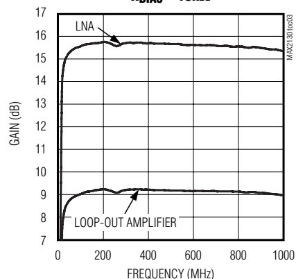
GAIN vs. FREQUENCY R BIAS = 10kΩ
