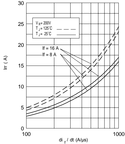
Fig. 6 - Typical Recovery Current vs. d i_f / dt , (per Leg)
