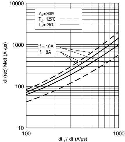
Fig. 8 - Typical d i_{(rec)} M / dt vs. d i_f / dt , (per Leg)
