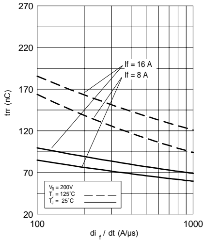
Fig. 5 - Typical Reverse Recovery vs. d i_f / dt , (per Leg)
