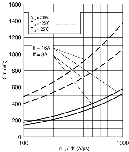
Fig. 7 - Typical Stored Charge vs. d i_f / dt , (per Leg)
