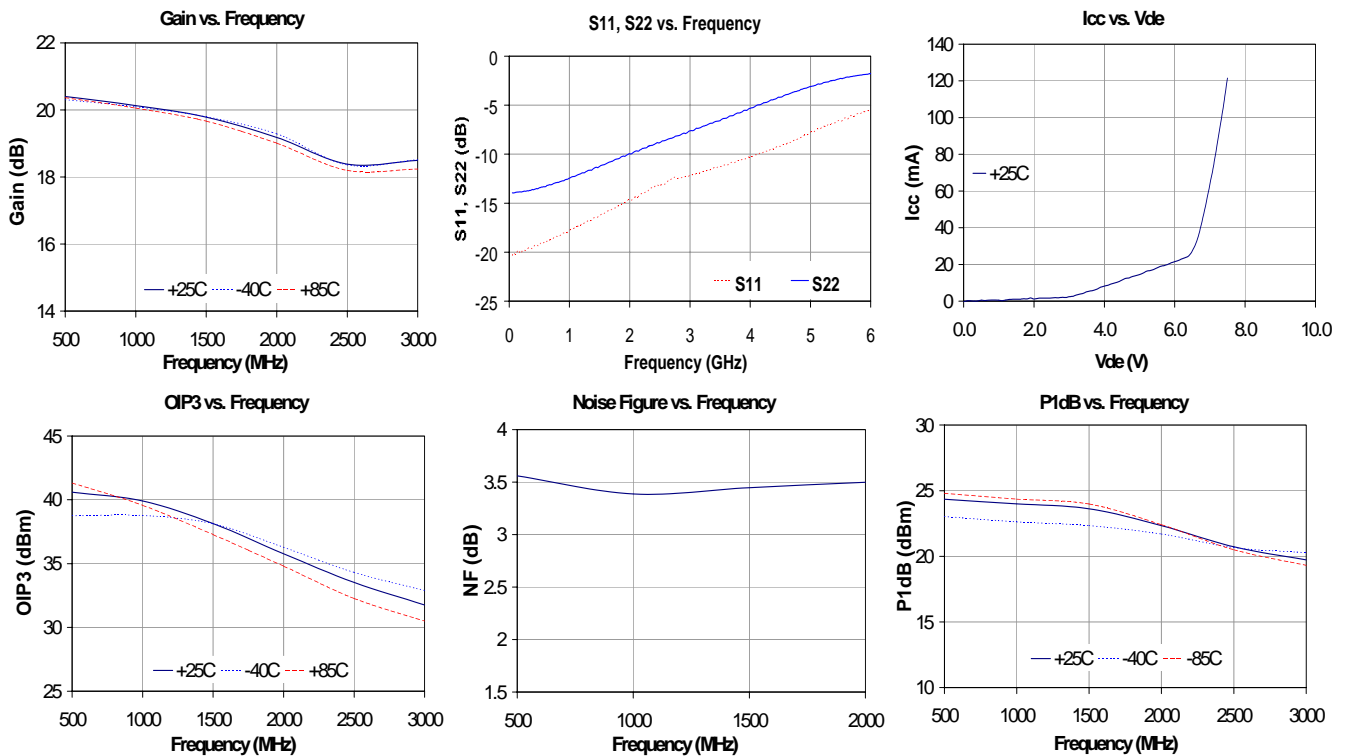
S-Parameters ( V_{device} = +7.2 \text{ V} , I_{cc} = 110 \text{ mA} , T = 25^\circ \text{C} , calibrated to device leads)
