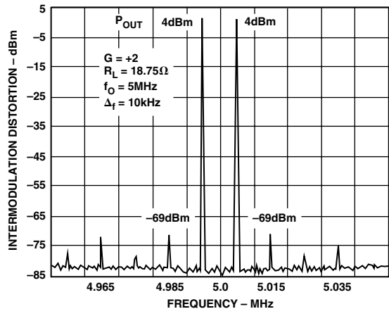
Figure 9. Intermodulation Distortion
