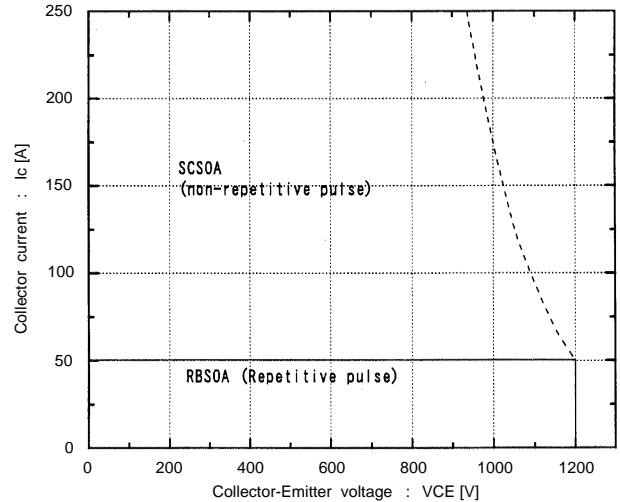
Reversed biased safe operating area +V_{GE}=15V, -V_{GE} \le 15V, T_J \le 125^\circ C, R_G \ge 51 \text{ ohm}
