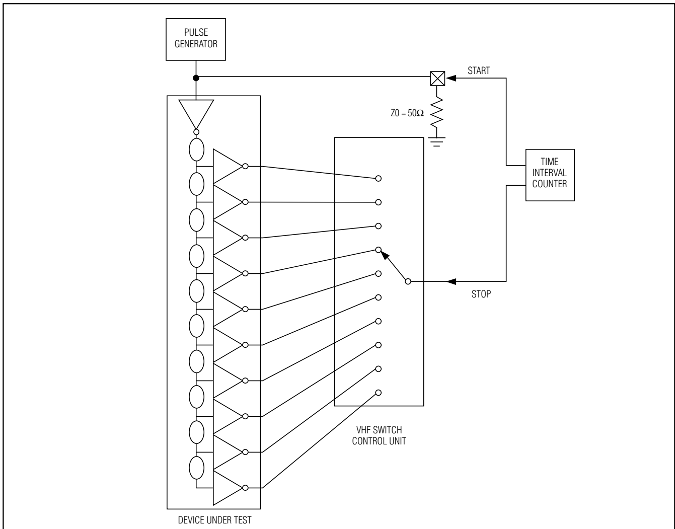
Figure 3. Test Circuit
