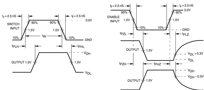
FIGURE 3. AC Waveforms
