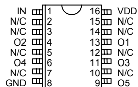
3D7205S SOL (300 Mil)
