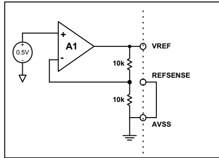
Figure 7: VREF=1V
