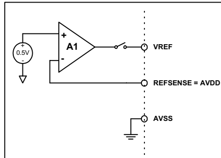
Figure 8: VREF=Hi Impedance
