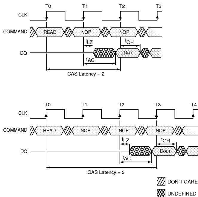
Figure 6 CAS Latency
