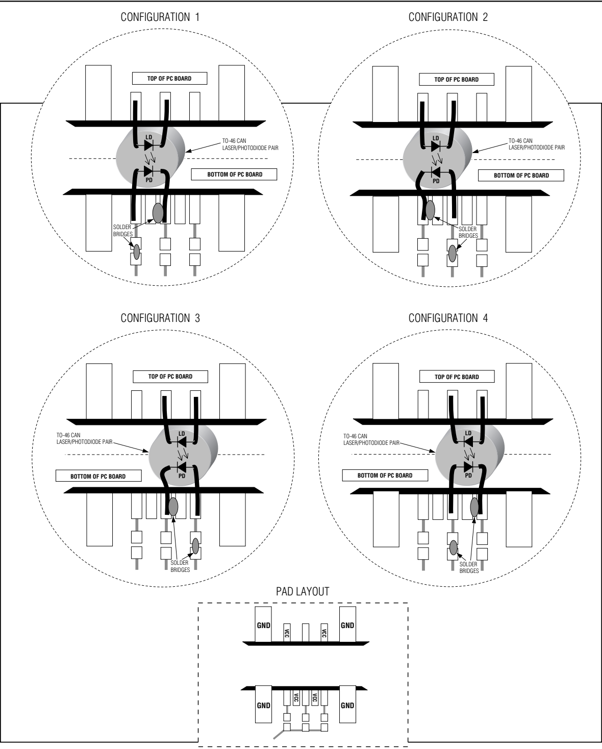
Figure 2. Attachment of a Laser Diode/Monitor Diode to the MAX3865 EV Kit
