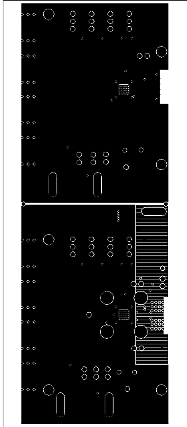
Figure 8. MAX3865 EV Kit PC Board Layout—Power Plane
