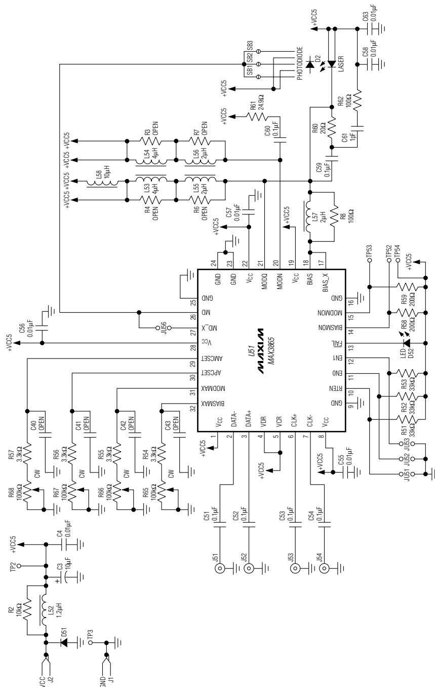
Figure 4. MAX3865 EV Kit Optical Board Schematic
