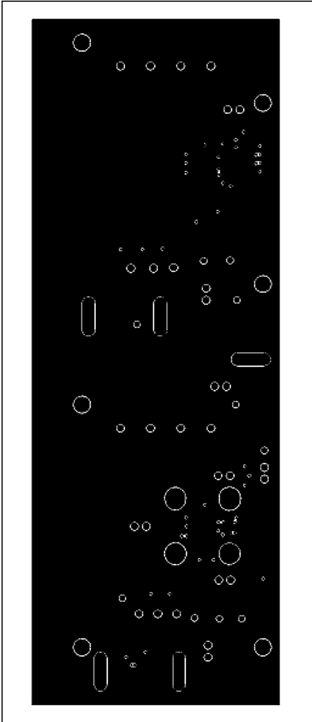
Figure 7. MAX3865 EV Kit PC Board Layout—Ground Plane
