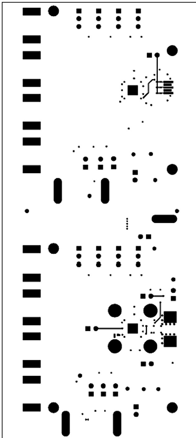
Figure 9. MAX3865 EV Kit PC Board Layout—Solder Side
