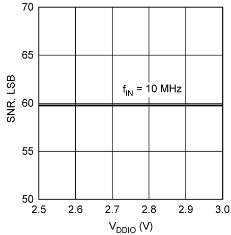
SNR vs. V_{DDIO}
