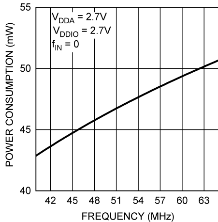
Power Consumption vs. f_{CLK}
