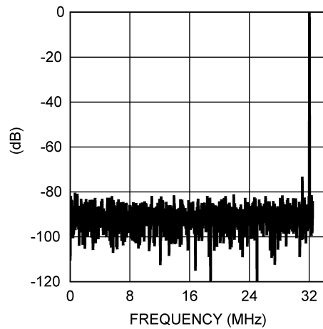
Spectral Response @ 32 MHz Input
