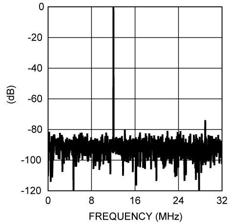
Spectral Response @ 11 MHz Input
