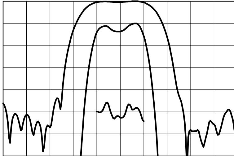
Horizontal: 0.5 MHz/div Vertical (from top): Magnitude 10 dB/div Magnitude 1 dB/div Group Delay 50 ns/div
