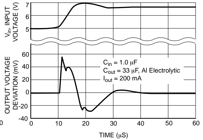
Figure 11. Line Transient
