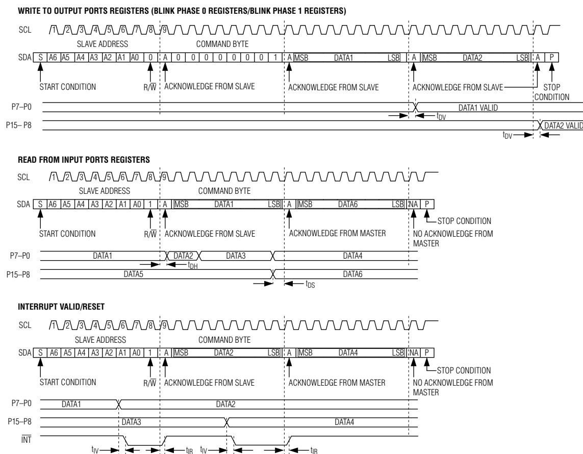
Figure 10. Read, Write, and Interrupt Timing Diagrams
