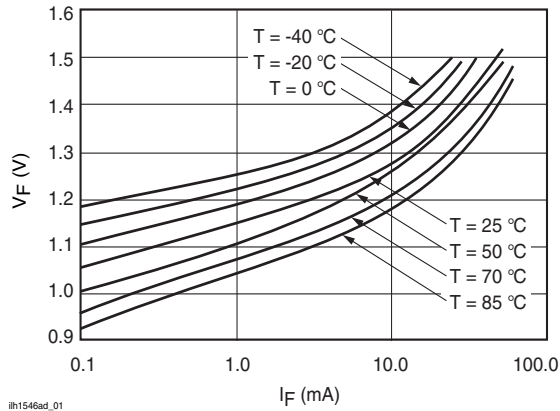
Fig. 2 LED Voltage vs. Temperature
