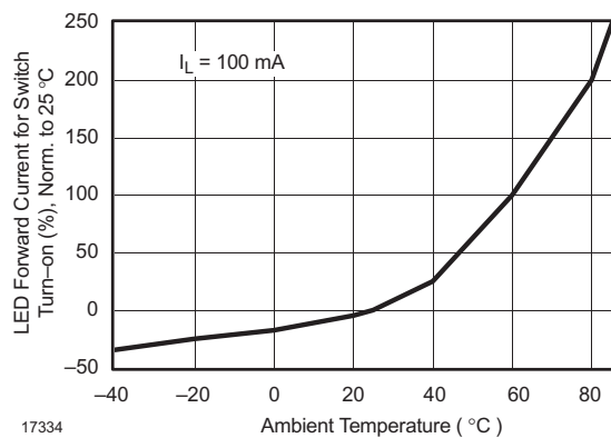
Fig. 3 LED Current for Switch Turn-on vs. Temperature
