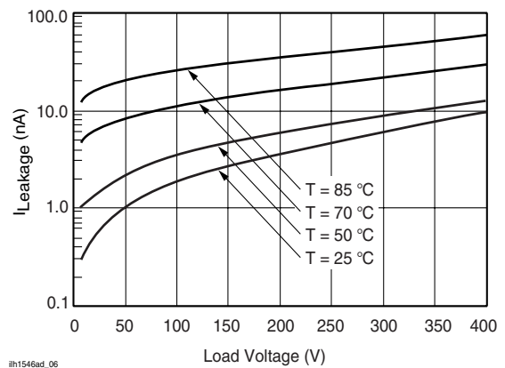
Fig. 6 Leakage Current vs. Applied Voltage
