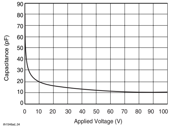
Fig. 5 Switch Capacitance vs. Applied Voltage
