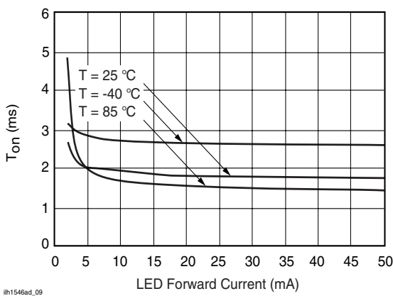
Fig. 9 Turn-on Time vs. LED Current
