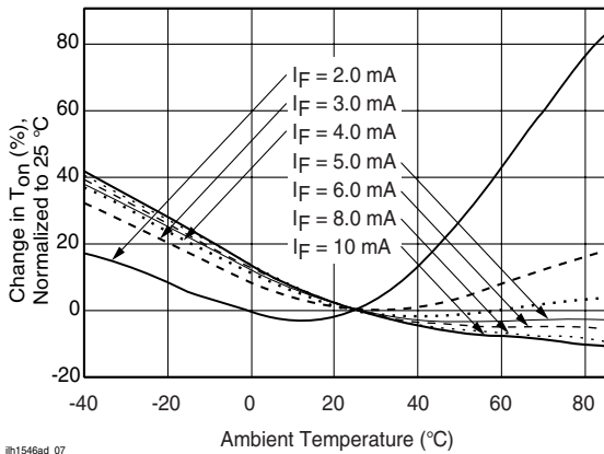
Fig. 7 Turn-on Time vs. Temperature
