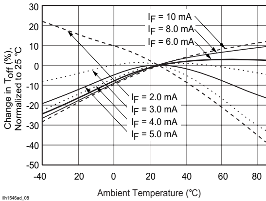
Fig. 8 Turn-off Time vs. Temperature
