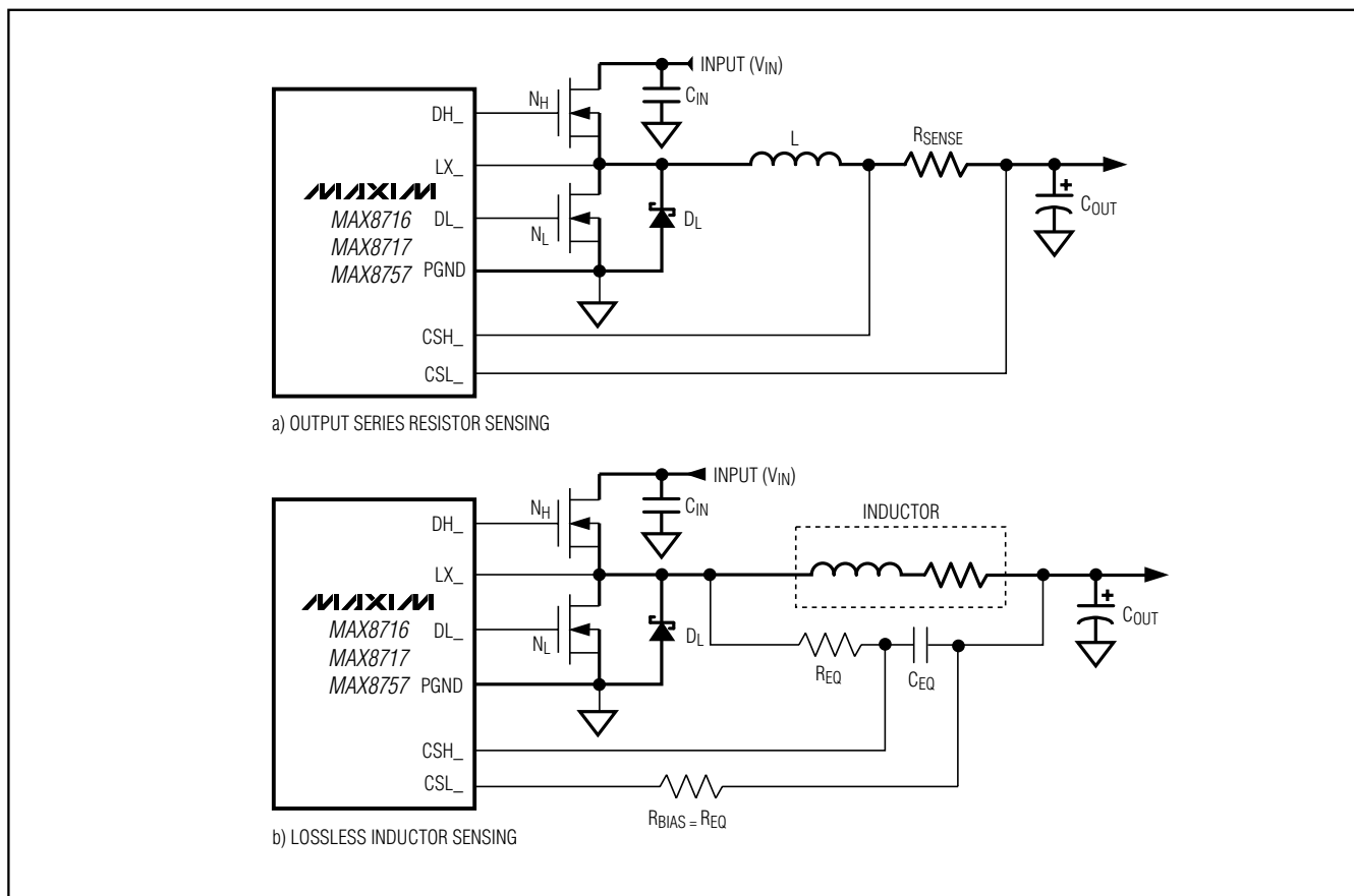
Figure 8. Current-Sense Configurations
