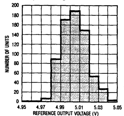
Distribution of Reference Output Voltage
