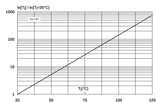
Fig. 6: Relative variation of leakage current versus junction temperature (typical values).
