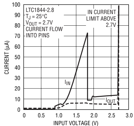
Figure 8. Reverse Current vs Input Voltage
