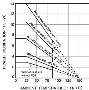
Fig.7 Thermal derating curves
