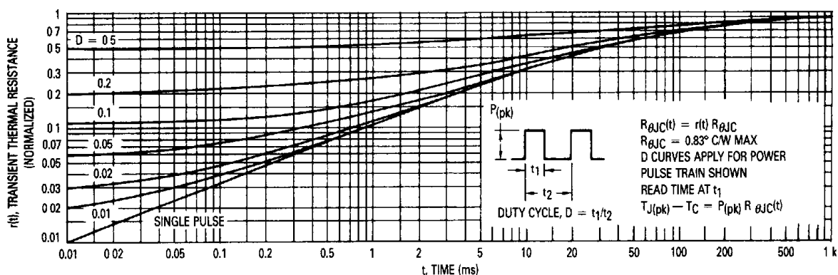
Figure 10. Thermal Response
