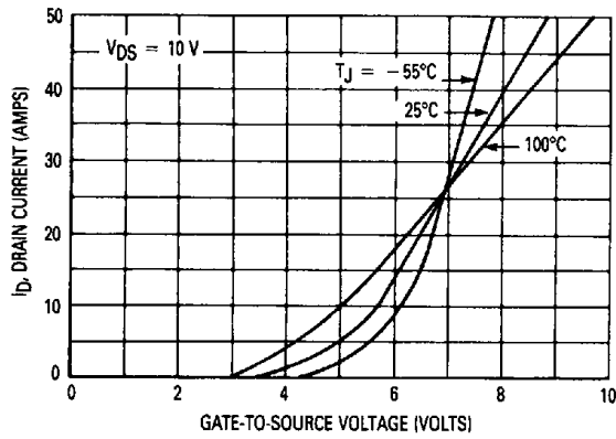
Figure 3. Transfer Characteristics
