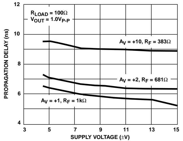
FIGURE 24. PROPAGATION DELAY vs SUPPLY VOLTAGE
