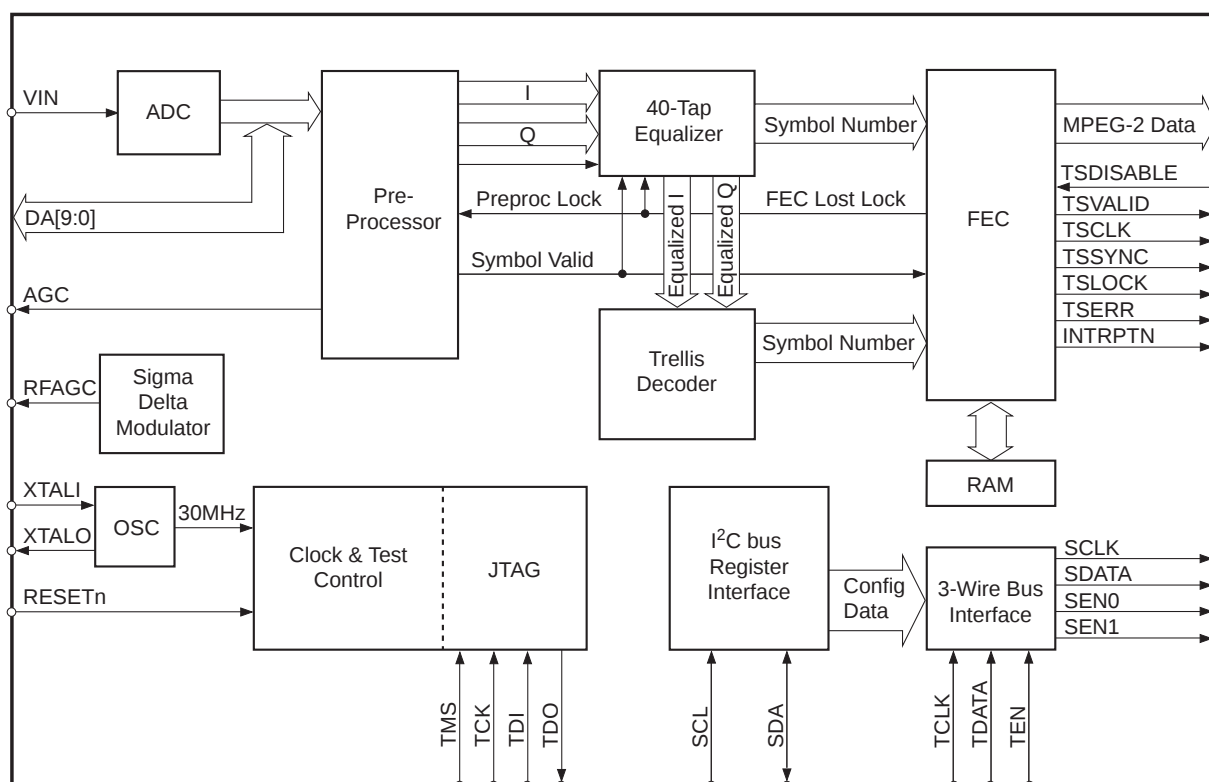
Fig. 2. Block Diagram
