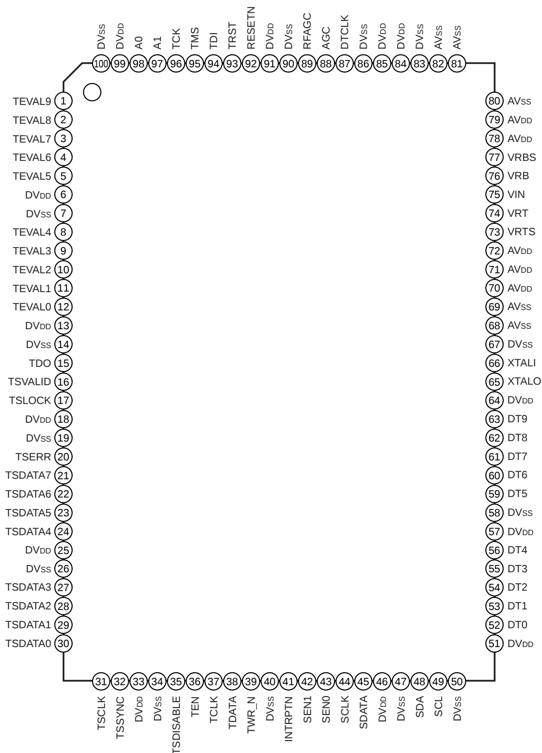
Fig. 1. Pin Configuration
