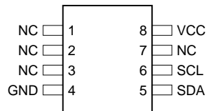
8-lead SOIC, PDIP or LAP
