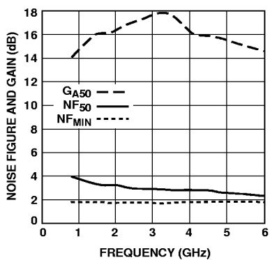
Figure 5. Gain and Noise Figure (50 \Omega Source and Load) vs. Frequency.
