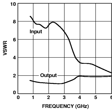
Figure 13. Input and Output VSWR vs. Frequency.
