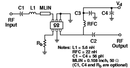
Figure 22. Schematic of 1.9 GHz Circuit.
