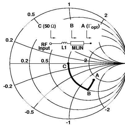
Figure 20. Input Impedance Match.
