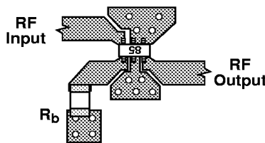
Figure 18. RF Layout.
