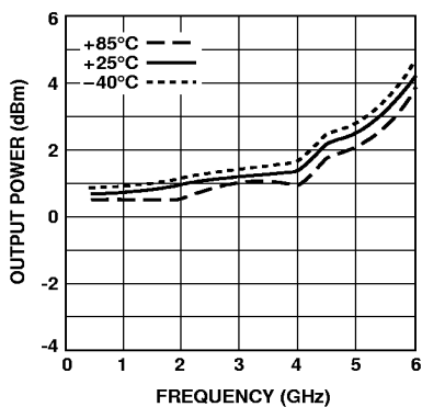
Figure 7. Output Power @ 1 dB Gain Compression vs. Frequency and Temperature.
