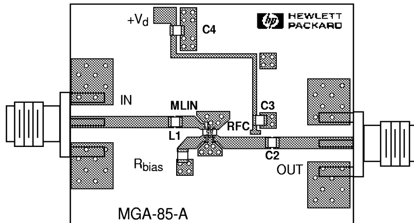
Figure 23. Complete 1.9 GHz Amplifier Circuit.
