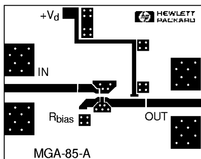
Figure 19. Multi-purpose PCB Layout.
