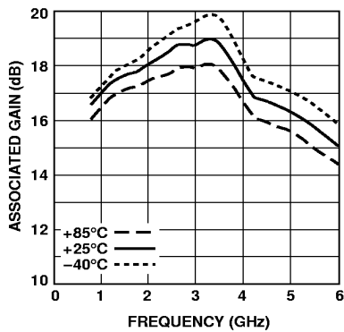
Figure 4. Associated Gain vs. Frequency and Temperature.
