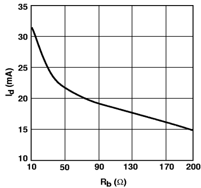
Figure 16. Bias Current vs. Resistor Value.
