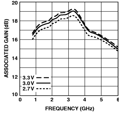
Figure 2. Associated Gain vs. Frequency and Voltage.
