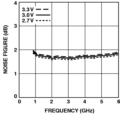
Figure 1. Minimum Noise Figure vs. Frequency and Voltage.
