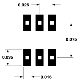
Figure 17. PCB Pad Layout for MGA-85563 Package (dimensions in inches).
