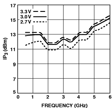
Figure 8. Output Third Order Intercept Point vs. Frequency and Voltage.
