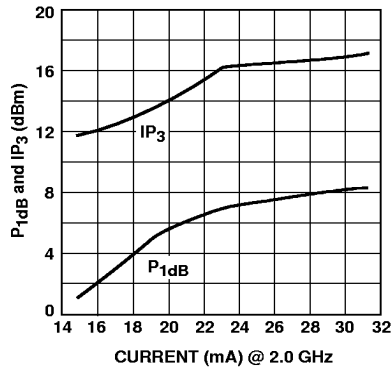
Figure 11. Output Third Order Intercept and P1dB vs. Device Current.
