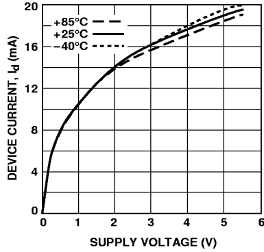
Figure 10. Device Current vs. Voltage and Temperature.
