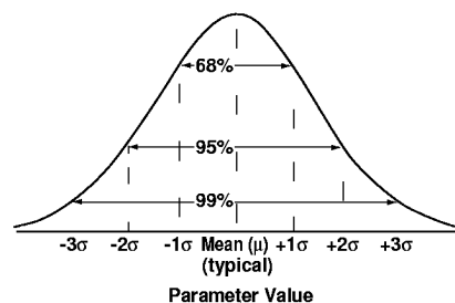
Figure 24. Normal Distribution.
