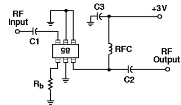
Figure 15. Schematic Diagram with Bias and Current Setting Connections.
