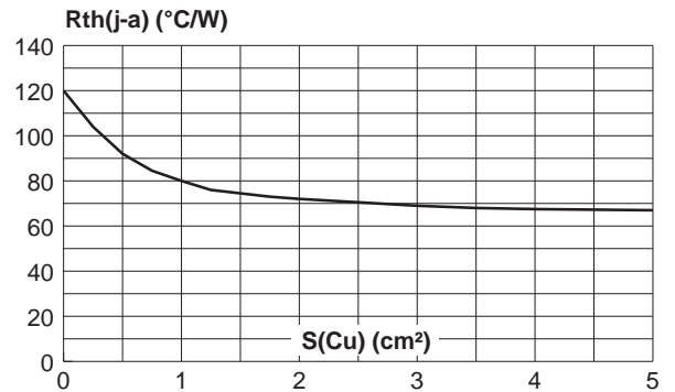
Fig. 10: Thermal resistance junction to ambient versus copper surface under each lead (Epoxy printed circuit board FR4, copper thickness: 35μm).
