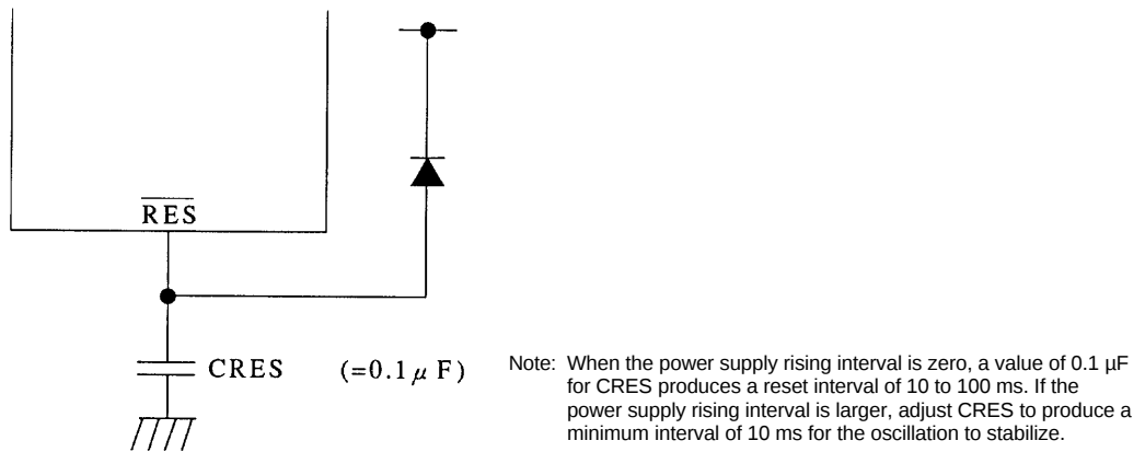
Figure 6 Reset Circuit
