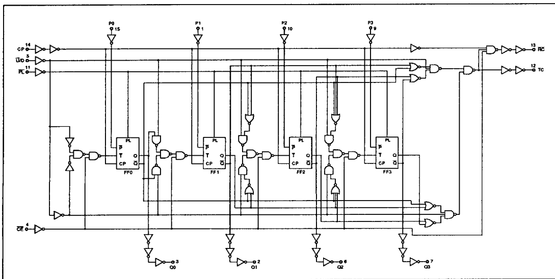
Figure 5: Logic Diagram
