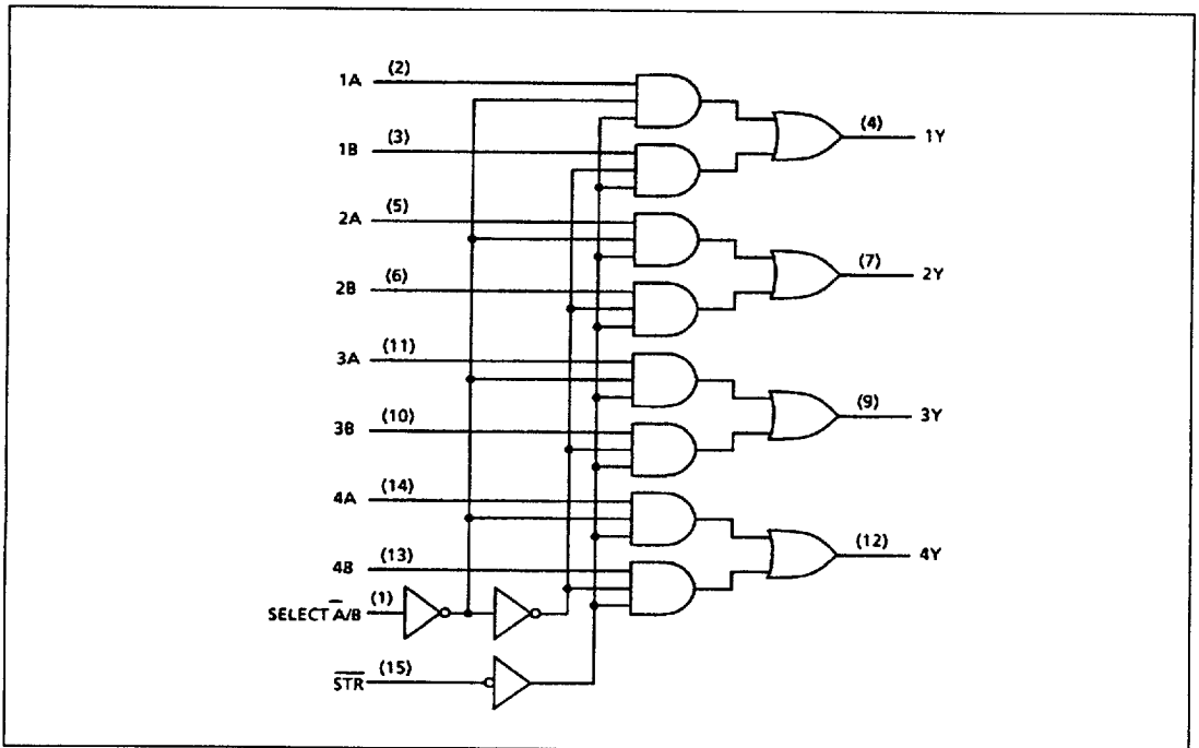
Figure 5: Logic Diagram
