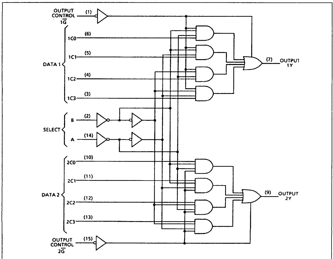
Figure 5: Logic Diagram
