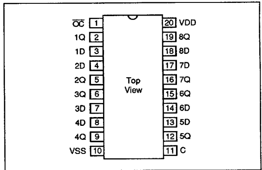
Figure 2: Pin Out
