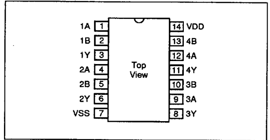
Figure 3: Pin Out
