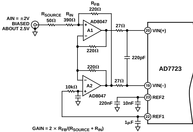
Figure 32. Single-Ended to Differential Input Circuit for Bipolar Mode Operation (Analog Input Biased About +2.5 V)
