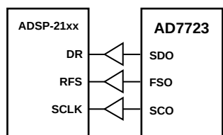
Figure 41. AD7723-to-ADSP-21xx Interface
