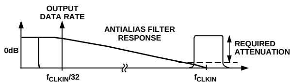
Figure 27b. Frequency Response of Antialias Filter
