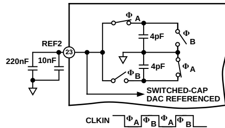
Figure 35. REF2 Equivalent Input Circuit
