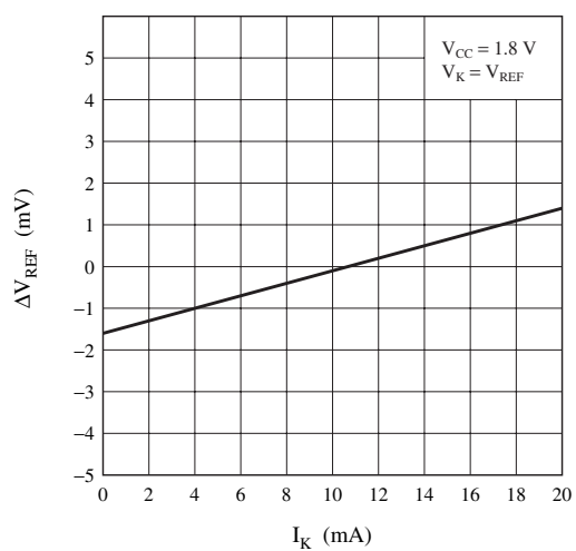
Reference voltage cathode current fluctuation
