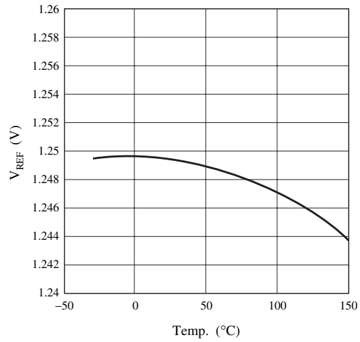
V_{REF} temperature characteristic
