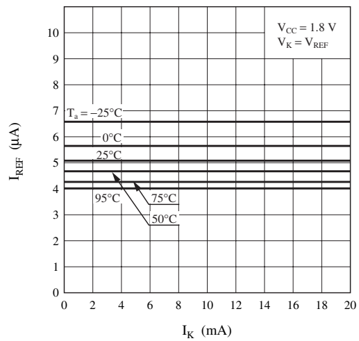
Reference current (temperature characteristics)
