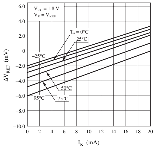
Reference voltage (temperature characteristics)
