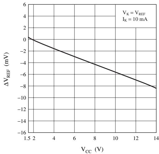
Reference voltage supply voltage fluctuation
