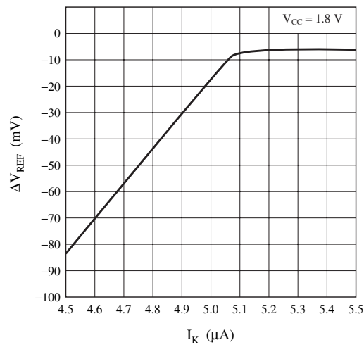
Minimum cathode current
