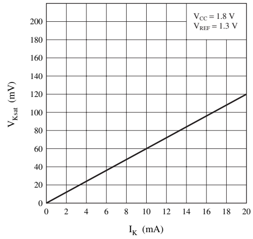
Cathode saturation voltage
