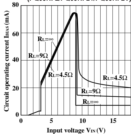
Fig.18 Circuit Operating Current vs. Input Voltage (PQ09RF2/PQ09RF21/PQ09RF2V)
